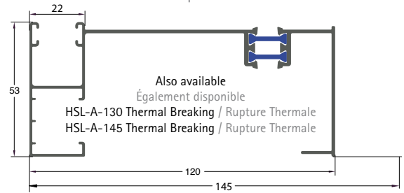
• HSL-A-120 Thermal Breaking Rupture Thermale
